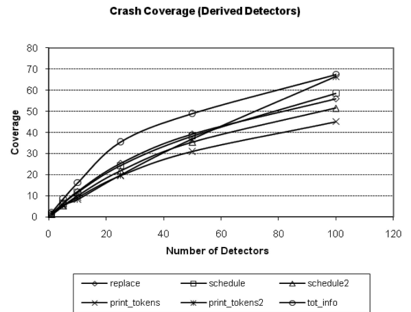
Fig. 5. Crash coverage of derived detectors.
