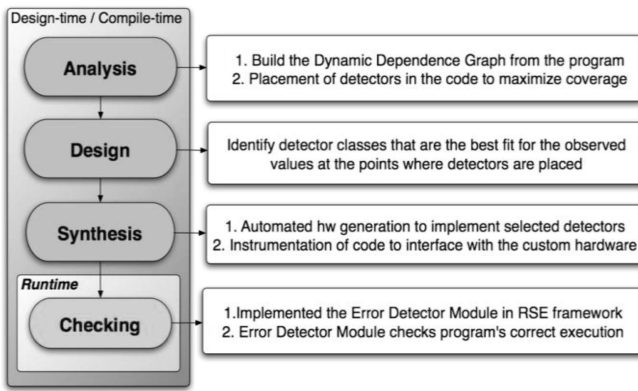
Fig. 1. Steps in detector derivation process.
