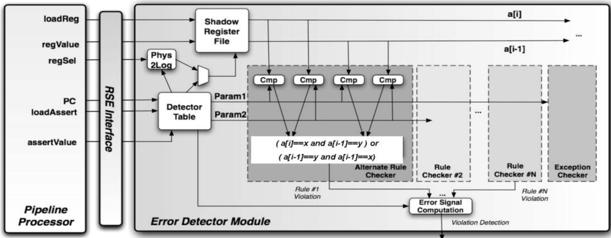
Fig. 4. Architectural diagram of synthesized processor.
