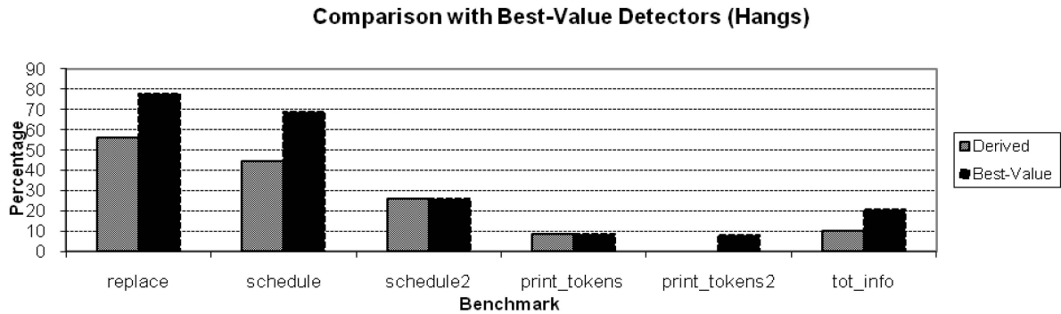
Fig. 16. Comparison between best-value detectors and derived detectors for hangs.
