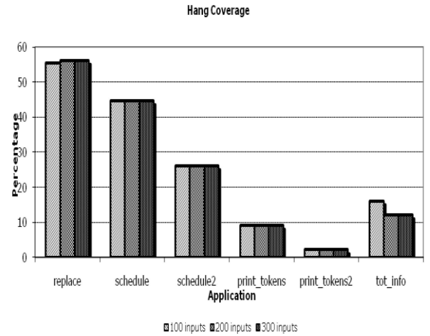
Fig. 12. Hang coverage for different training set sizes.
