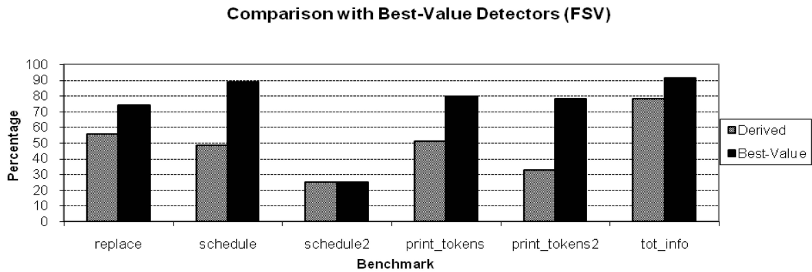
Fig. 15. Comparison between best-value detectors and derived detectors for FSV.
