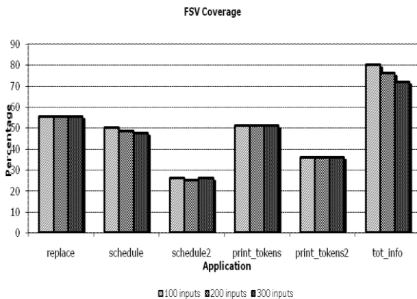
Fig. 11. FSV coverage for different training set sizes.
