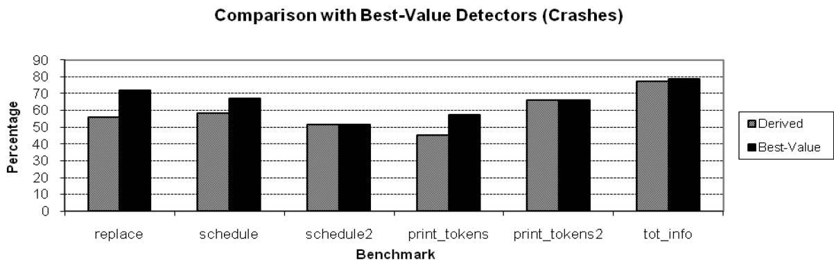
Fig. 14. Comparison between best-value detectors and derived detectors for crashes.
