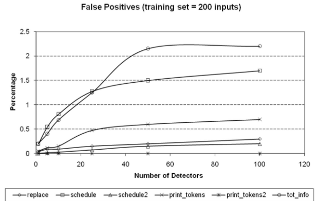
Fig. 9. Percentage of false positives for 1,000 inputs.
