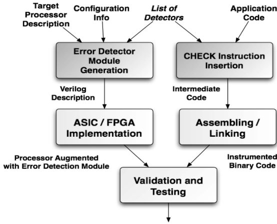
Fig. 2. Design flow to instrument application and generate the EDM from the list of detectors.
