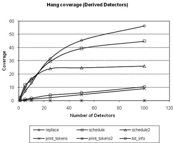
Fig. 7. Hang coverage of derived detectors.
