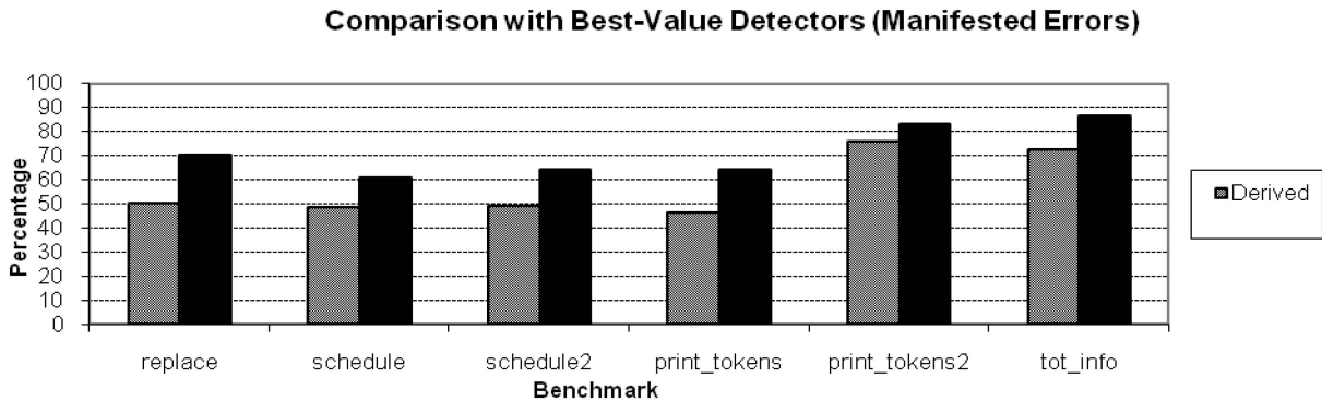
Fig. 17. Comparison between best-value detectors and derived detectors for manifested errors.
