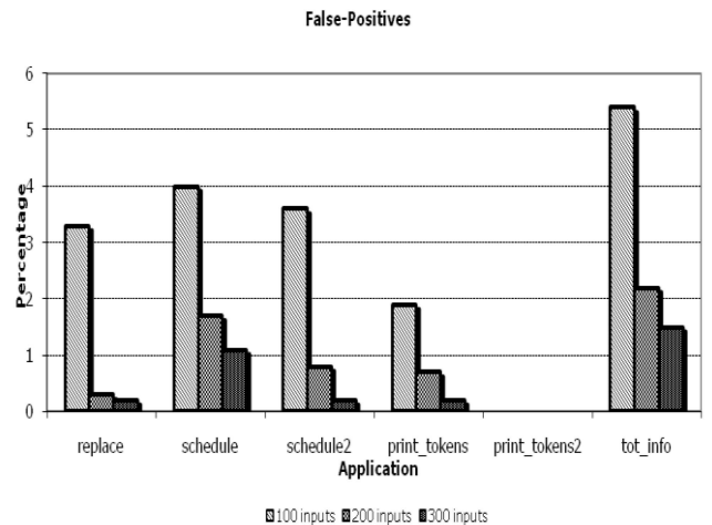
Fig. 13. False positives for different training set sizes.
