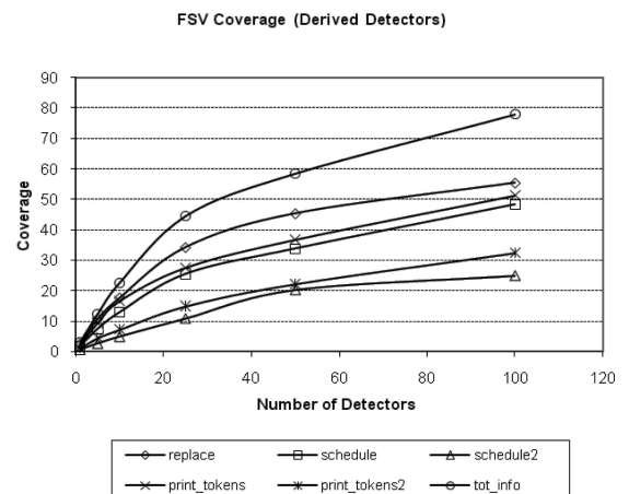
Fig. 6. FSV coverage of derived detectors.
