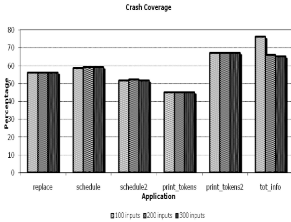
Fig. 10. Crash coverage for different training set sizes.
